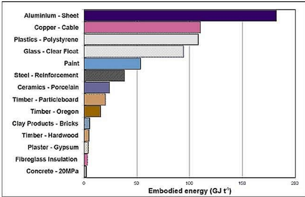
Figure 16 - Embodied Energy of Building Materials (Tucker, S., 2000)
