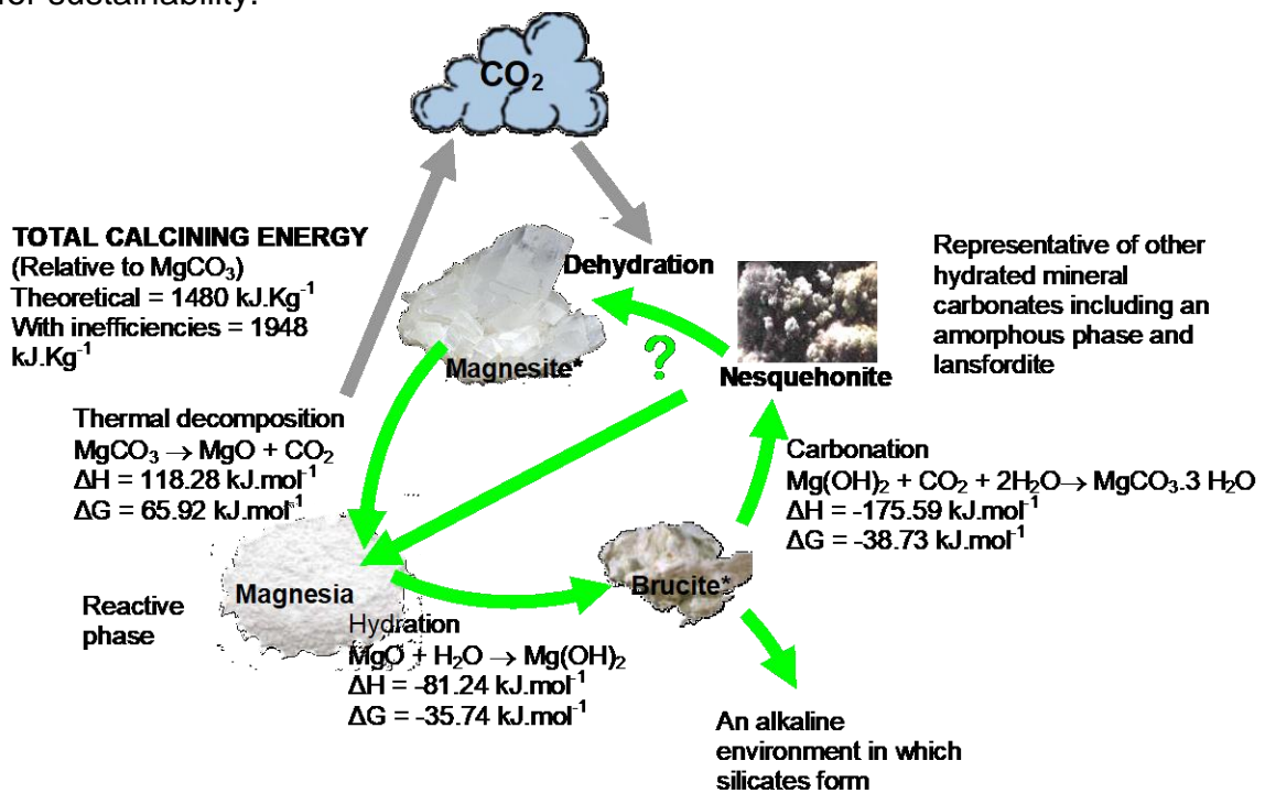
Figure 27 - The Magnesium Thermodynamic Cycle
