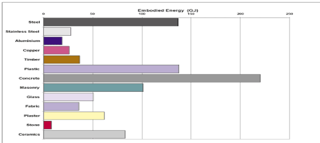
Figure 18 - Embodied Energy in Buildings (Tucker, S., 2000)
